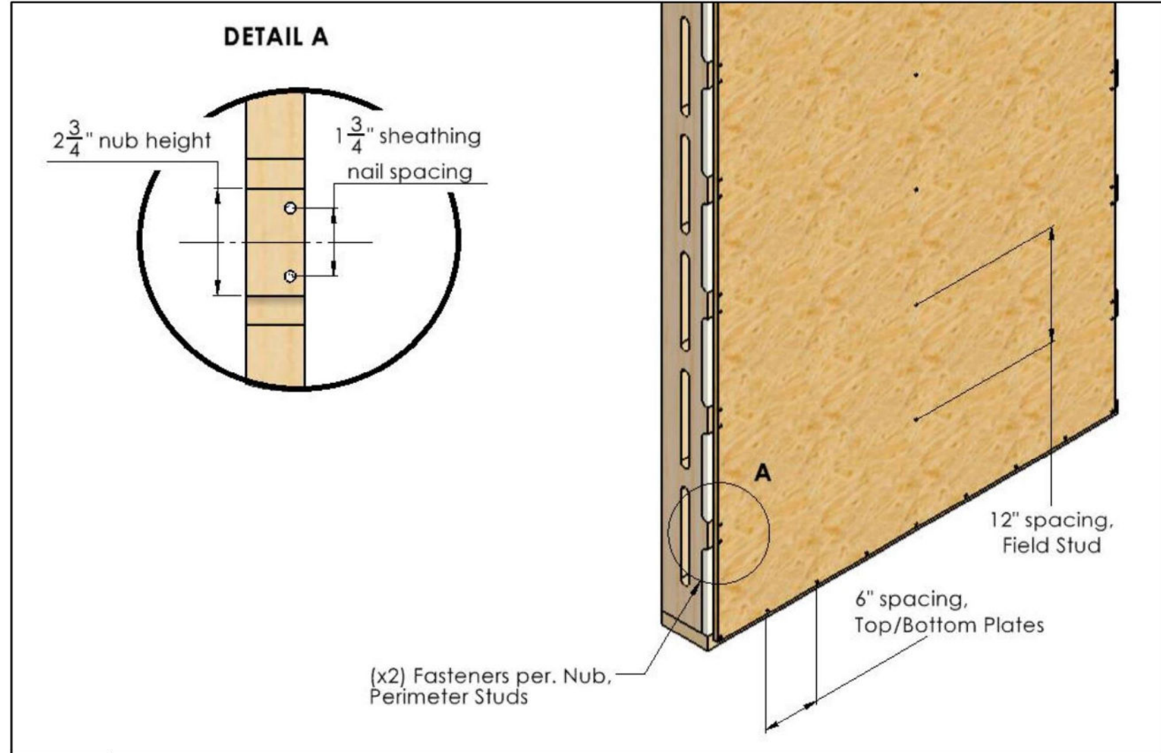
Figure 1: OSB Sheathing Nailing Pattern Diagram
